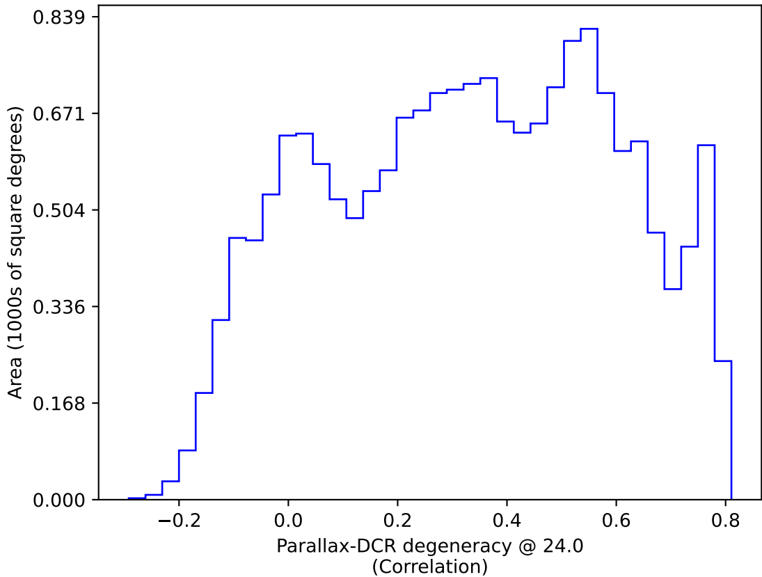
ddf_loaded_half_fl15_v3.4_10yrs WFD: Parallax-DCR degeneracy @ 24.0
