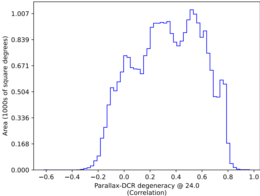
ddf_loaded_half_fl15_v3.4_10yrs All sky: Parallax-DCR degeneracy @ 24.0
