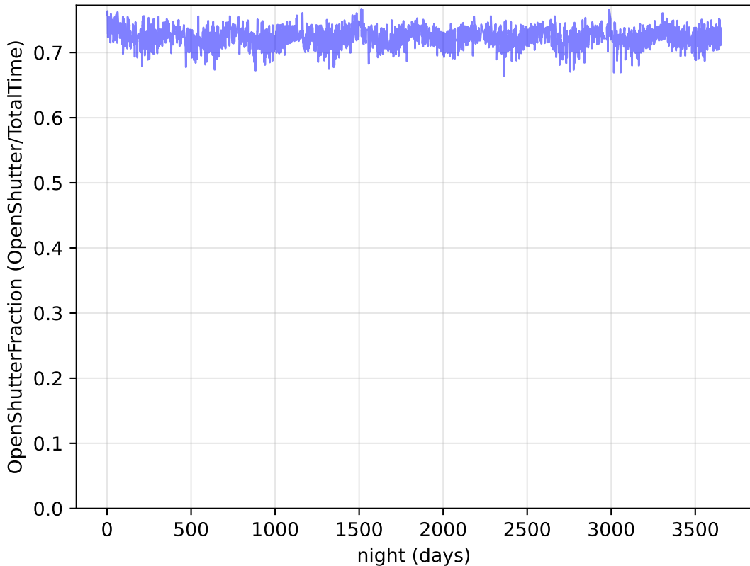
ddf_loaded_half_fl15_v3.4_10yrs Per night: OpenShutterFraction
