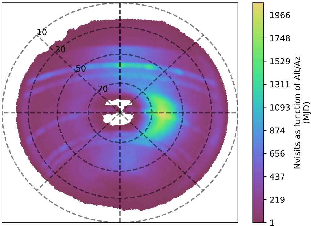
ddf_loaded_half_fl15_v3.4_10yrs z band: Nvisits as function of Alt/Az
