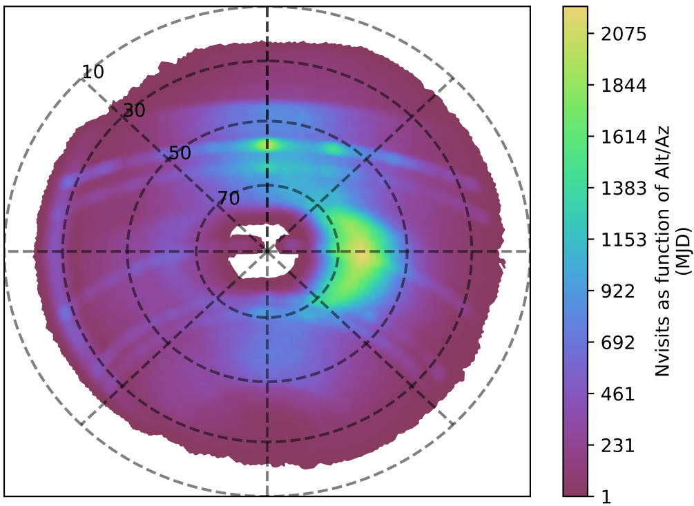
ddf_loaded_half_fl15_v3.4_10yrs r band: Nvisits as function of Alt/Az
