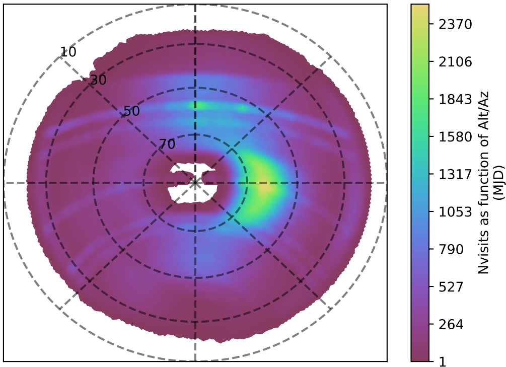
ddf_loaded_half_fl15_v3.4_10yrs i band: Nvisits as function of Alt/Az
