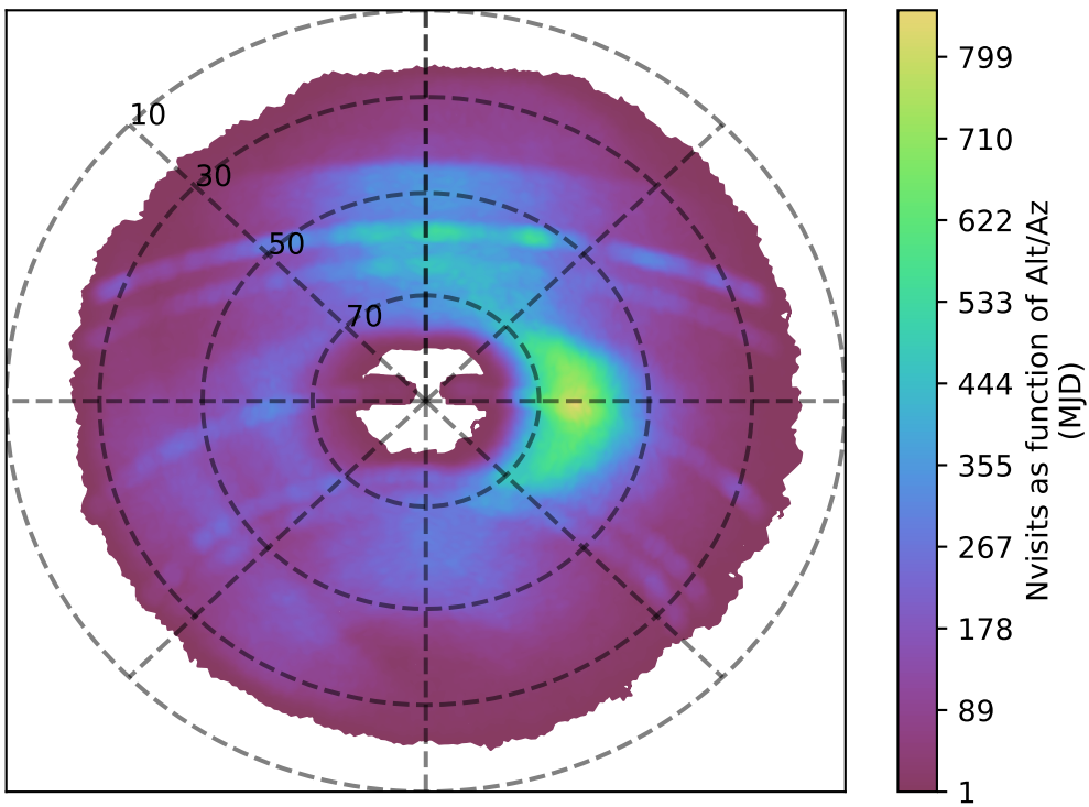
ddf_loaded_half_fl15_v3.4_10yrs g band: Nvisits as function of Alt/Az
