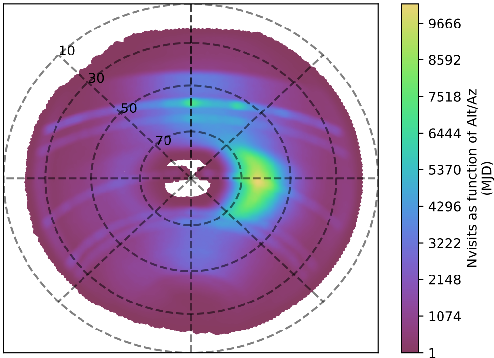
ddf_loaded_half_fl15_v3.4_10yrs all bands: Nvisits as function of Alt/Az
