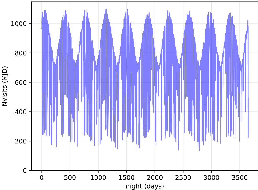
ddf_loaded_half_fl15_v3.4_10yrs All visits: Nvisits
