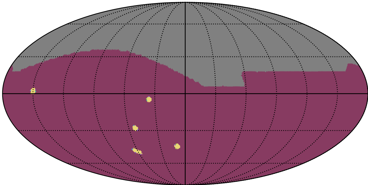
ddf_loaded_half_fl15_v3.4_10yrs All sky: NumberOfQuickRevisits
