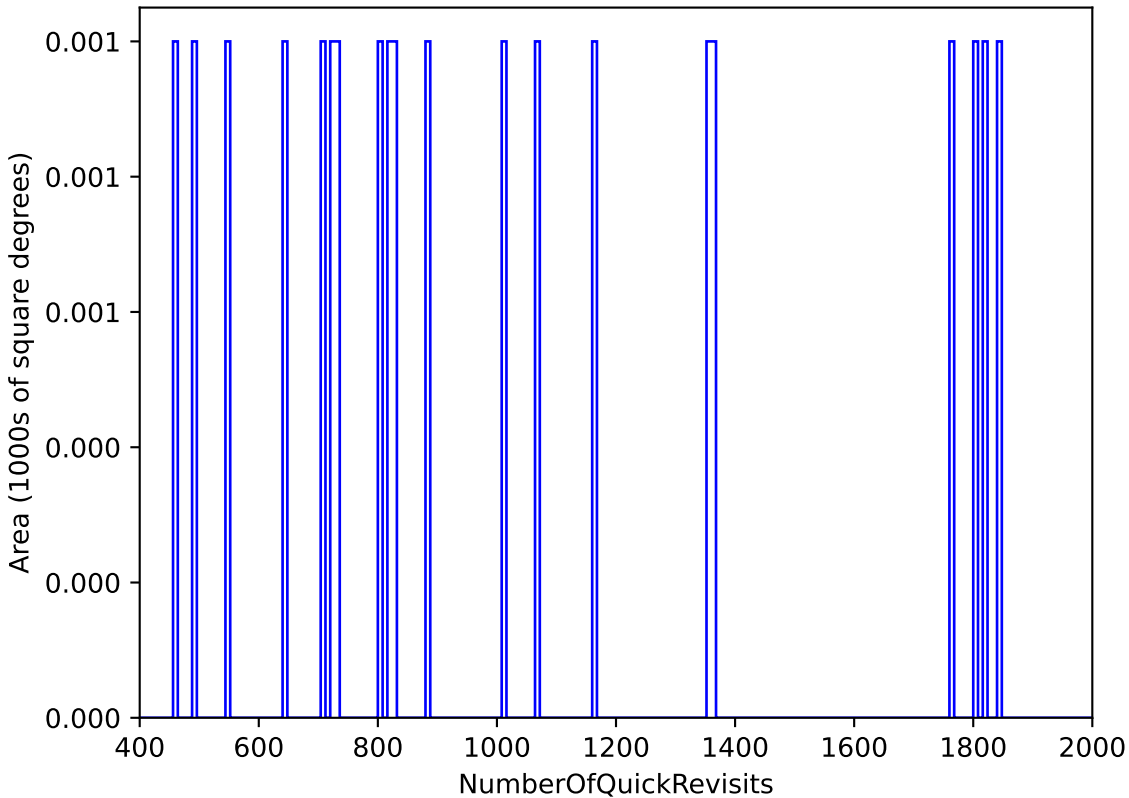
ddf_loaded_half_fl15_v3.4_10yrs All sky: NumberOfQuickRevisits
