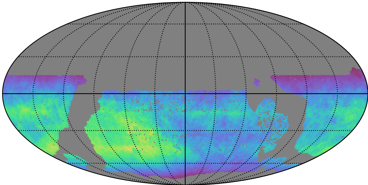
ddf_loaded_half_fl15_v3.4_10yrs WFD z band: Normalized Teff
