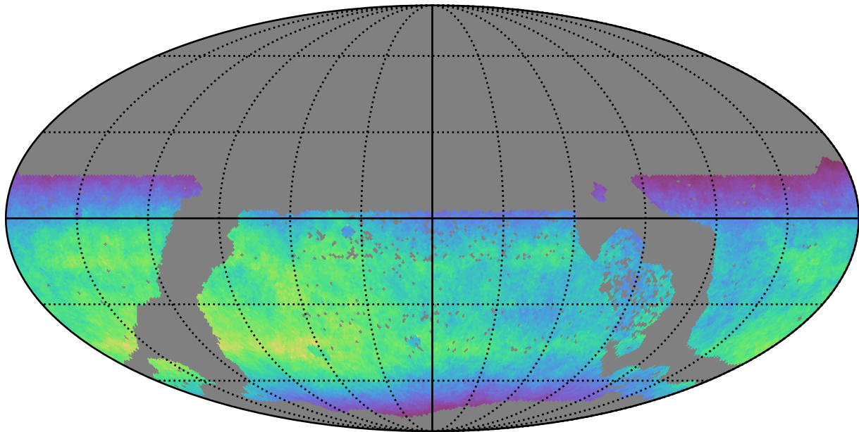
ddf_loaded_half_fl15_v3.4_10yrs WFD y band: Normalized Teff
