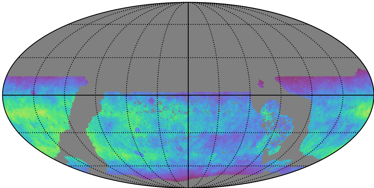
ddf_loaded_half_fl15_v3.4_10yrs WFD u band: Normalized Teff
