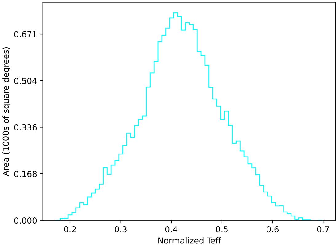
ddf_loaded_half_fl15_v3.4_10yrs WFD u band: Normalized Teff
