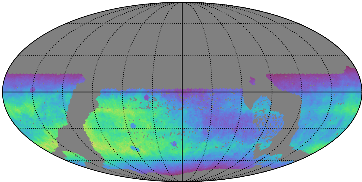
ddf_loaded_half_fl15_v3.4_10yrs WFD r band: Normalized Teff
