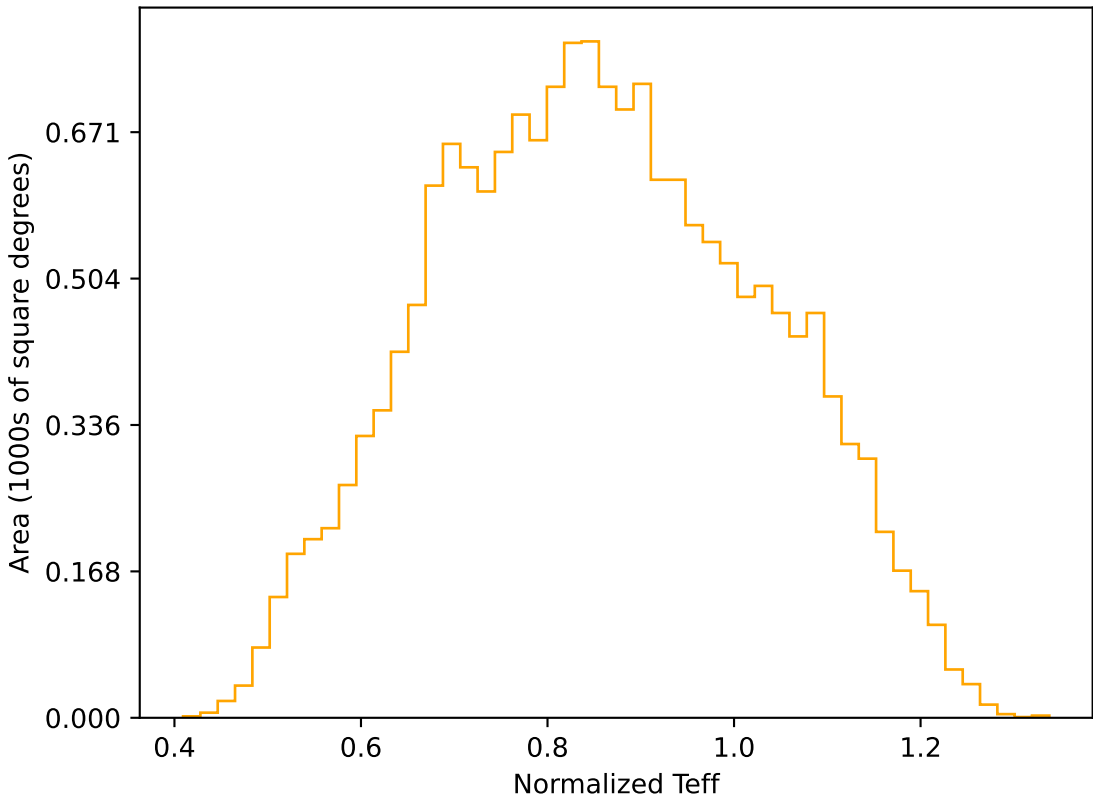
ddf_loaded_half_fl15_v3.4_10yrs WFD r band: Normalized Teff
