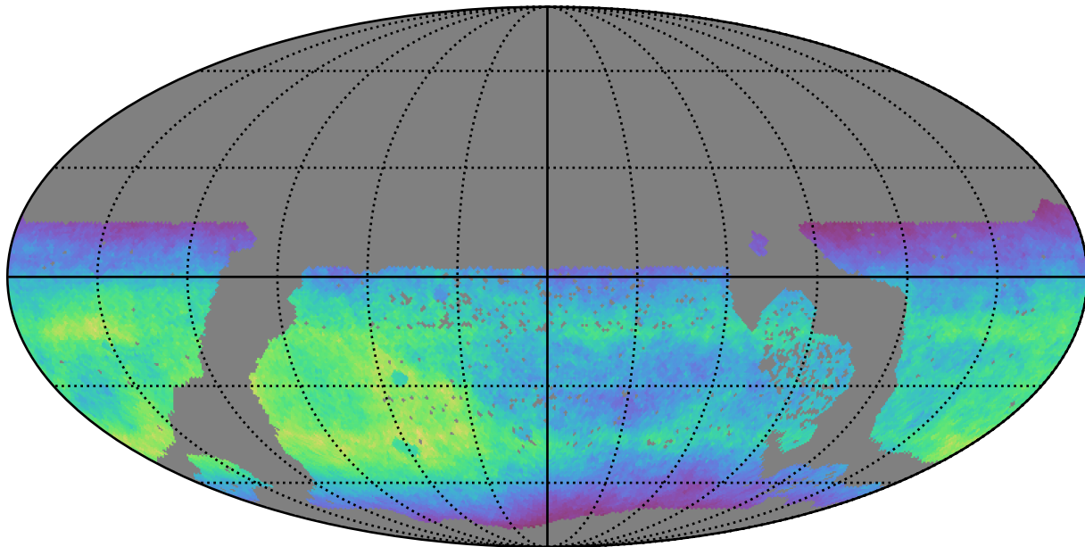
ddf_loaded_half_fl15_v3.4_10yrs WFD i band: Normalized Teff
