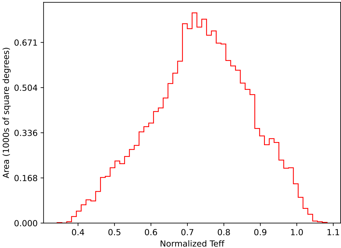
ddf_loaded_half_fl15_v3.4_10yrs WFD i band: Normalized Teff
