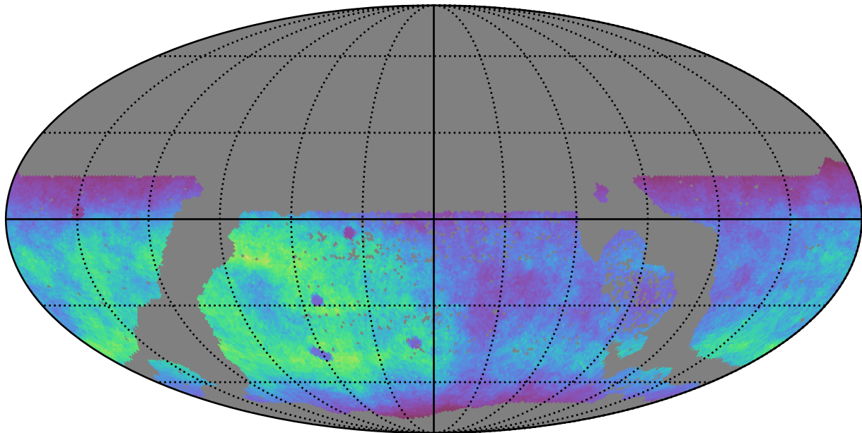
ddf_loaded_half_fl15_v3.4_10yrs WFD g band: Normalized Teff
