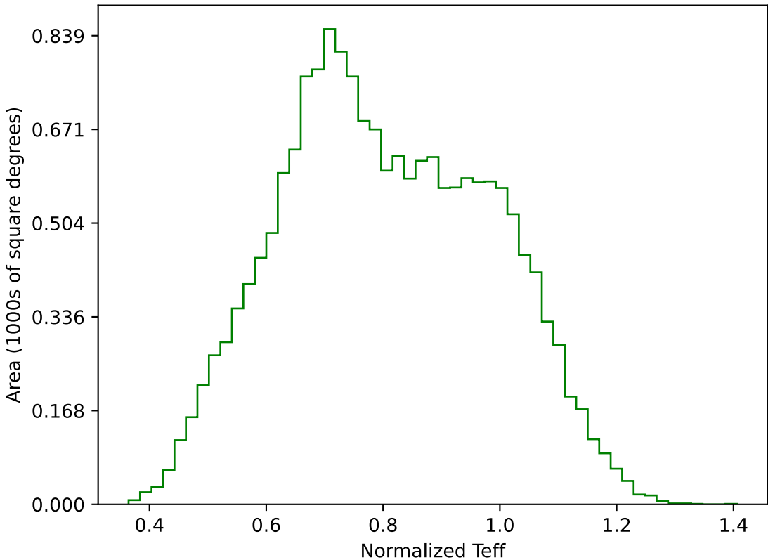
ddf_loaded_half_fl15_v3.4_10yrs WFD g band: Normalized Teff
