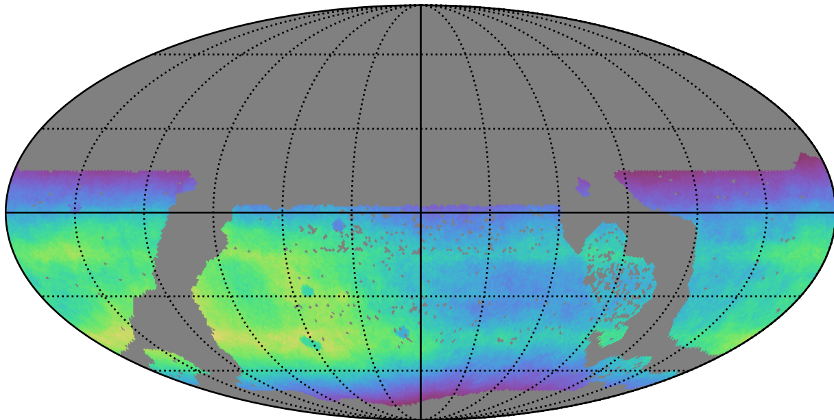
ddf_loaded_half_fl15_v3.4_10yrs WFD all bands: Normalized Teff
