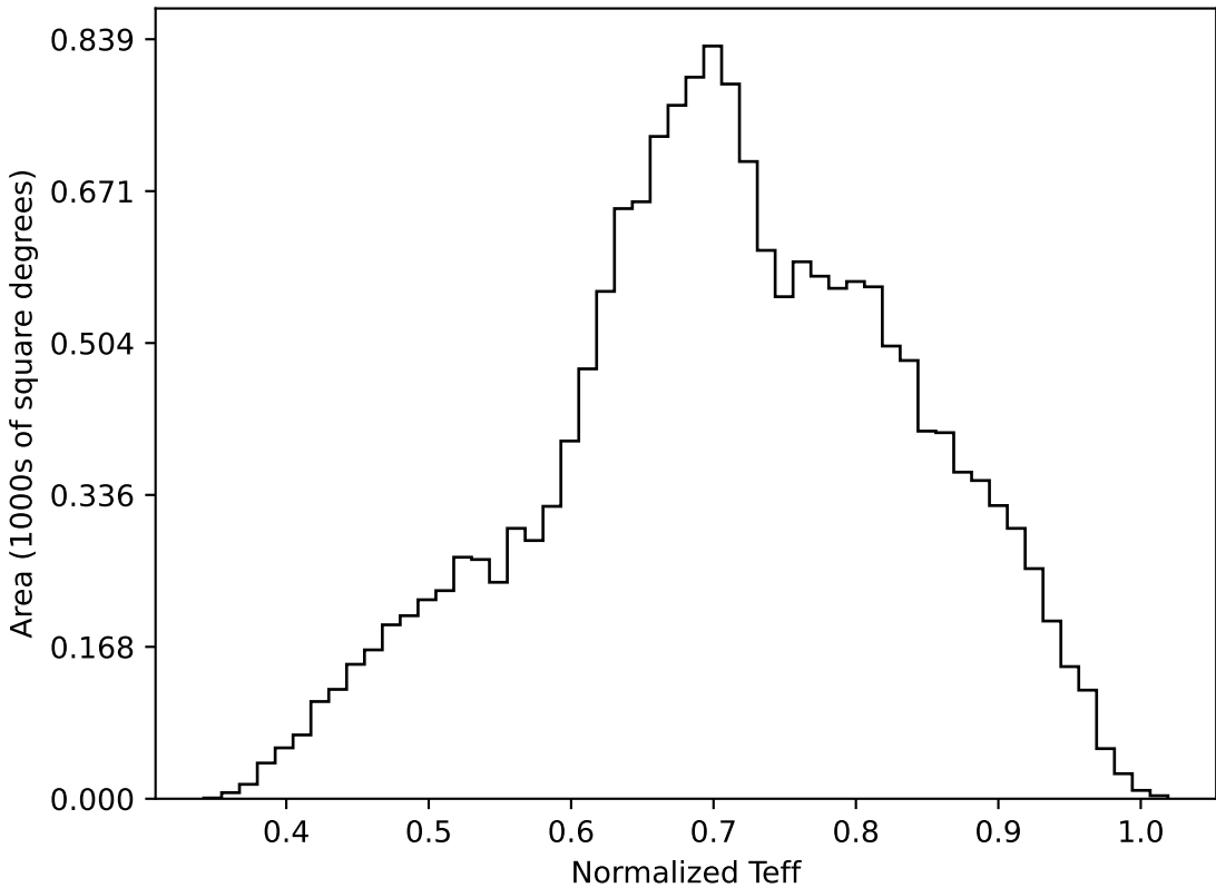
ddf_loaded_half_fl15_v3.4_10yrs WFD all bands: Normalized Teff
