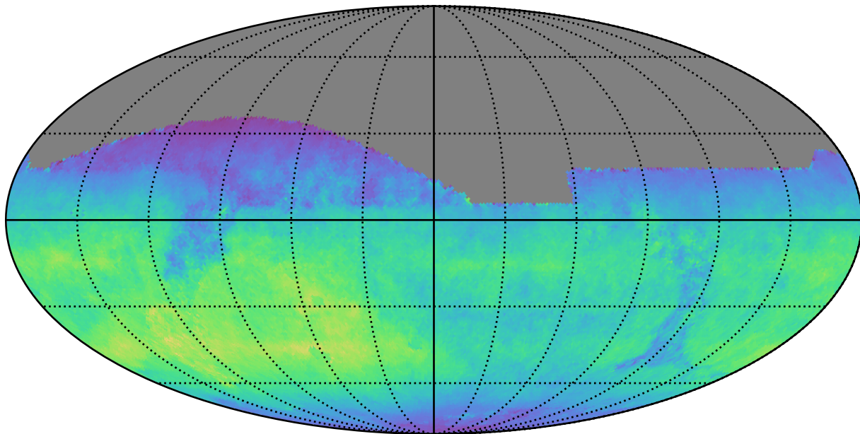
ddf_loaded_half_fl15_v3.4_10yrs All sky z band: Normalized Teff
