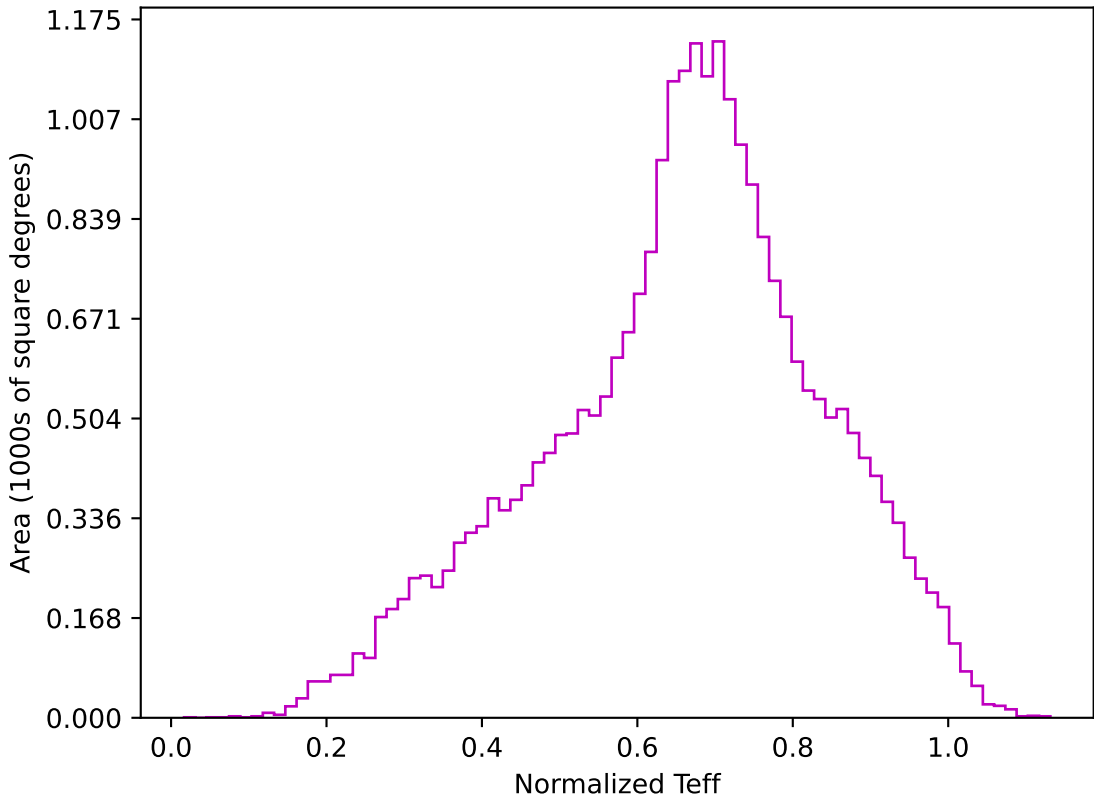
ddf_loaded_half_fl15_v3.4_10yrs All sky z band: Normalized Teff
