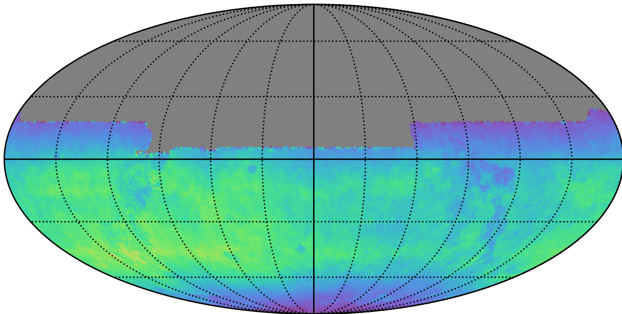
ddf_loaded_half_fl15_v3.4_10yrs All sky y band: Normalized Teff
