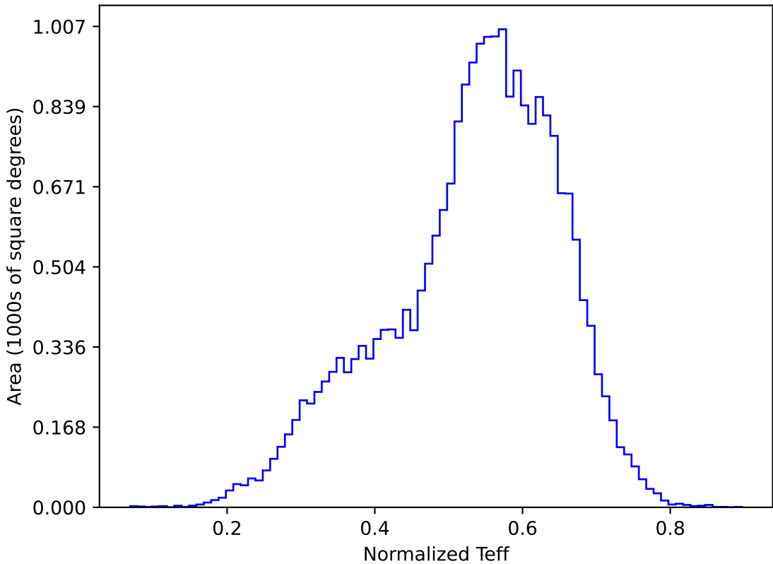
ddf_loaded_half_fl15_v3.4_10yrs All sky y band: Normalized Teff
