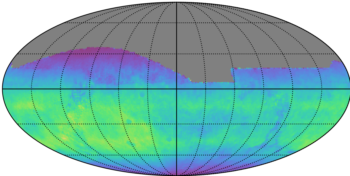
ddf_loaded_half_fl15_v3.4_10yrs All sky i band: Normalized Teff
