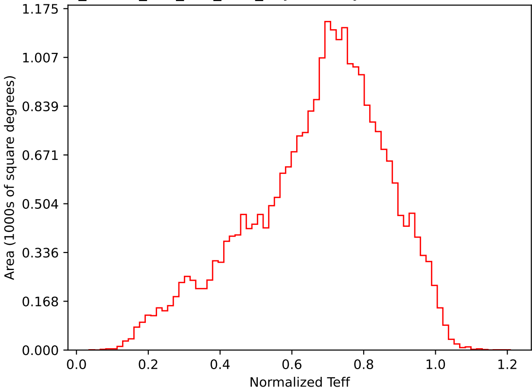
ddf_loaded_half_fl15_v3.4_10yrs All sky i band: Normalized Teff
