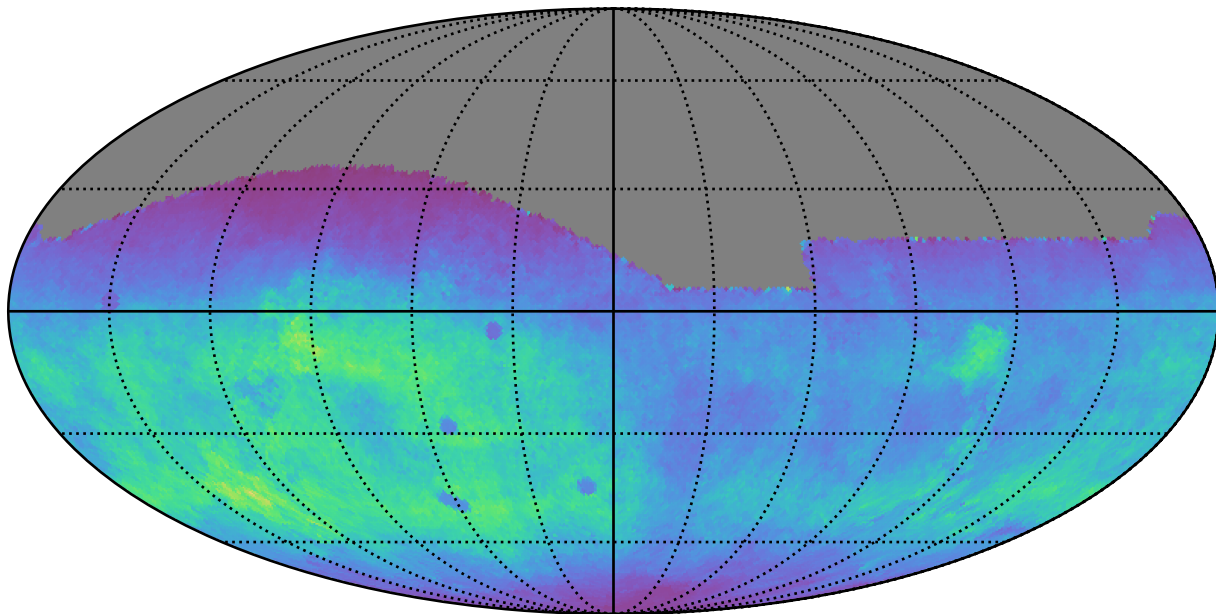
ddf_loaded_half_fl15_v3.4_10yrs All sky g band: Normalized Teff
