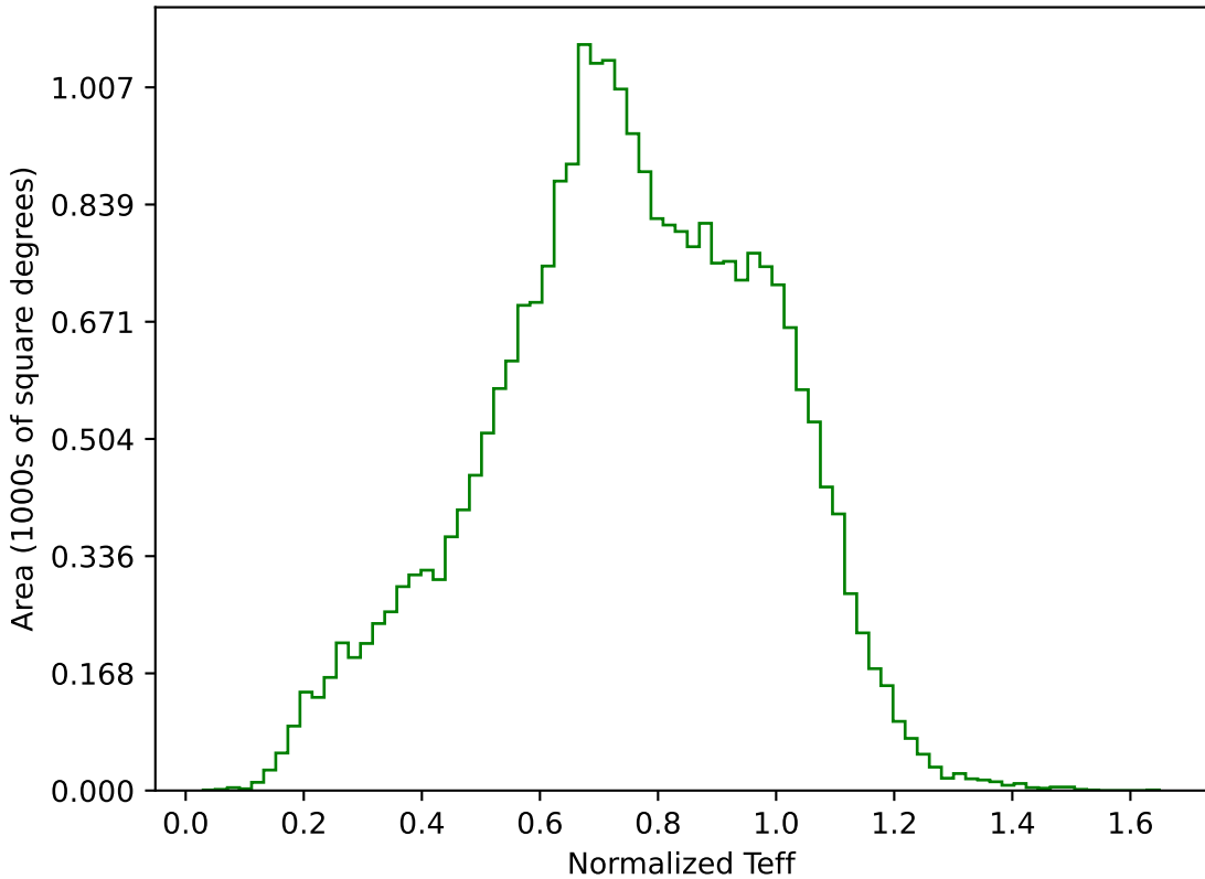
ddf_loaded_half_fl15_v3.4_10yrs All sky g band: Normalized Teff
