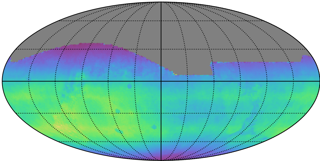
ddf_loaded_half_fl15_v3.4_10yrs All sky all bands: Normalized Teff
