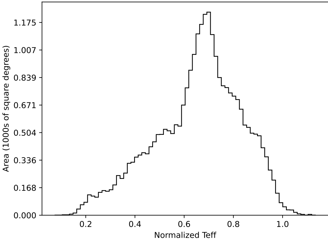
ddf_loaded_half_fl15_v3.4_10yrs All sky all bands: Normalized Teff
