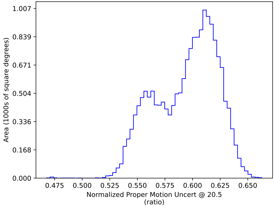
ddf_loaded_half_fl15_v3.4_10yrs WFD: Normalized Proper Motion Uncert @ 20.5
