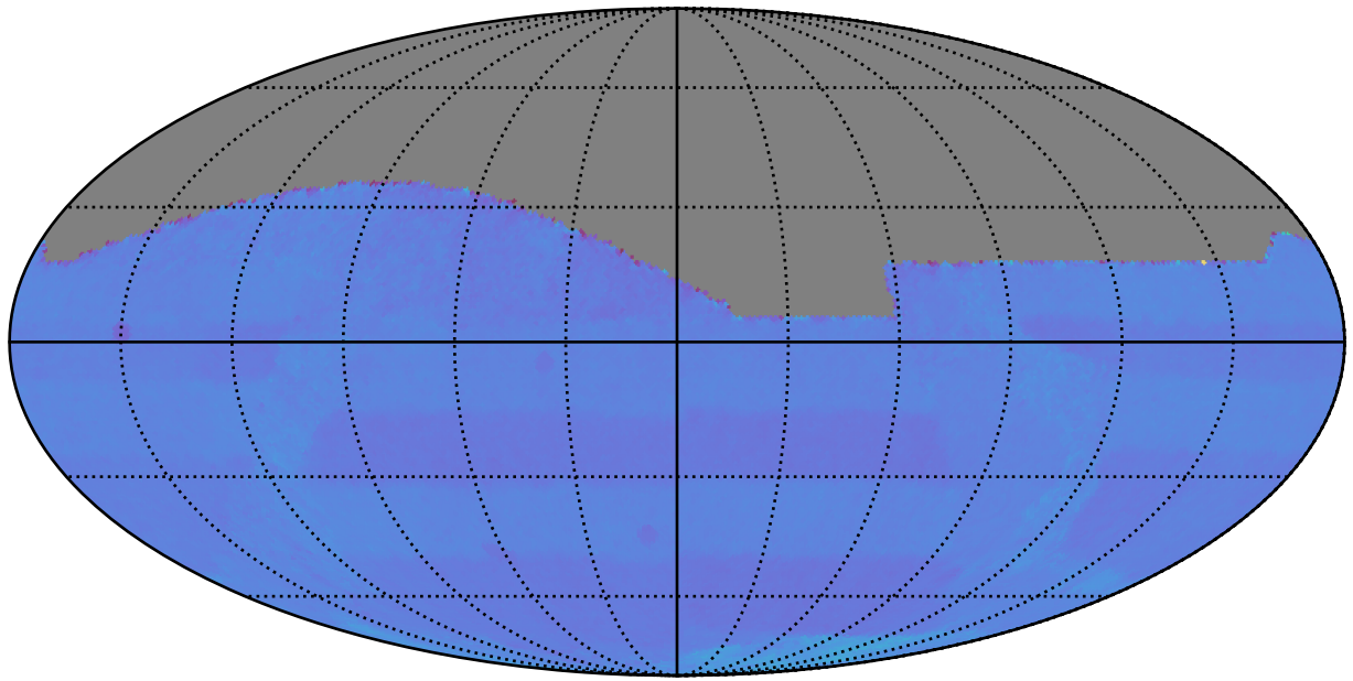
ddf_loaded_half_fl15_v3.4_10yrs All sky: Normalized Proper Motion Uncert @ 20.5
