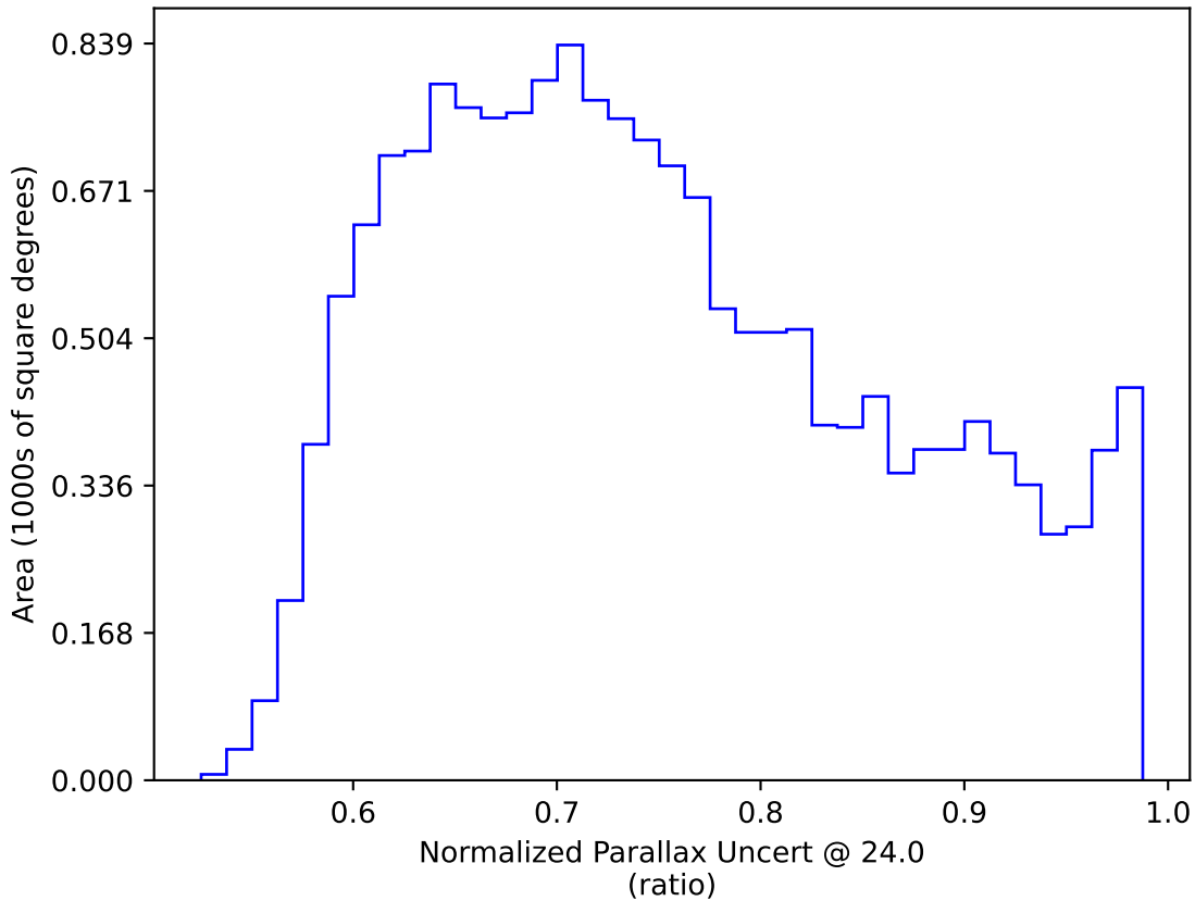
ddf_loaded_half_fl15_v3.4_10yrs WFD: Normalized Parallax Uncert @ 24.0
