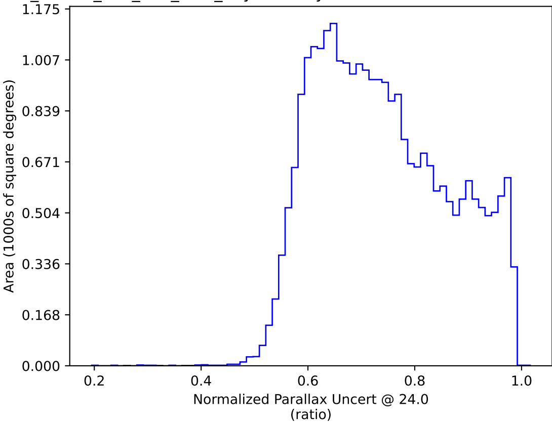
ddf_loaded_half_fl15_v3.4_10yrs All sky: Normalized Parallax Uncert @ 24.0
