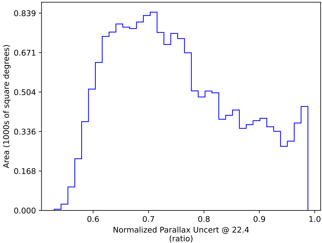
ddf_loaded_half_fl15_v3.4_10yrs WFD: Normalized Parallax Uncert @ 22.4
