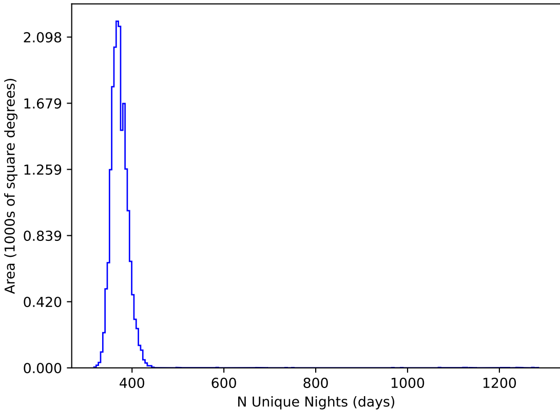
ddf_loaded_half_fl15_v3.4_10yrs WFD all bands: N Unique Nights
