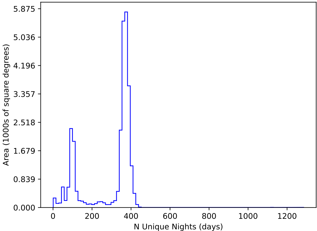
ddf_loaded_half_fl15_v3.4_10yrs All sky all bands: N Unique Nights
