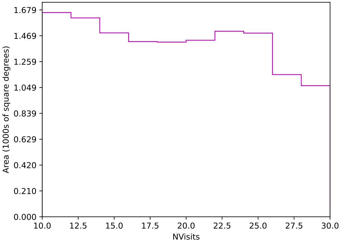
ddf_loaded_half_fl15_v3.4_10yrs Yr 3-4 z band: NVisits
