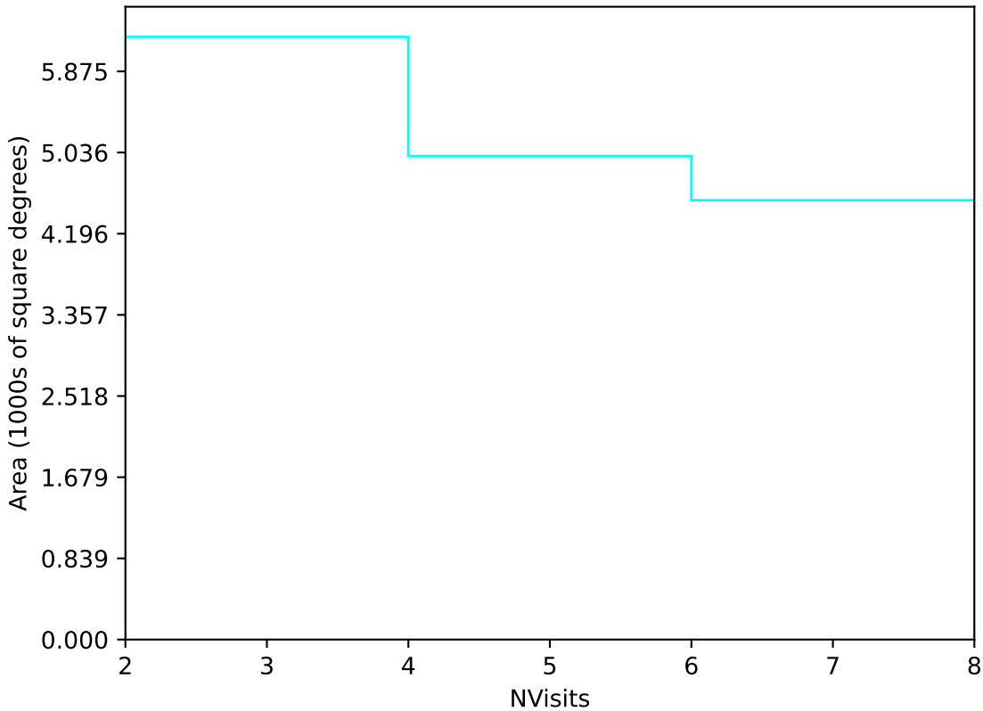
ddf_loaded_half_fl15_v3.4_10yrs Yr 3-4 u band: NVisits
