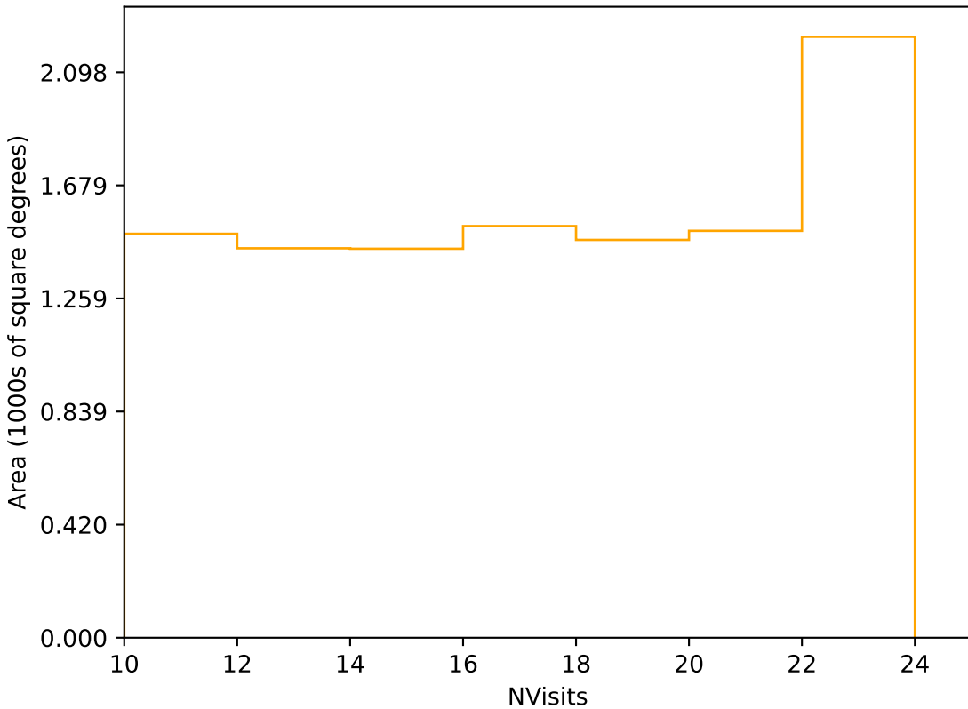
ddf_loaded_half_fl15_v3.4_10yrs Yr 3-4 r band: NVisits
