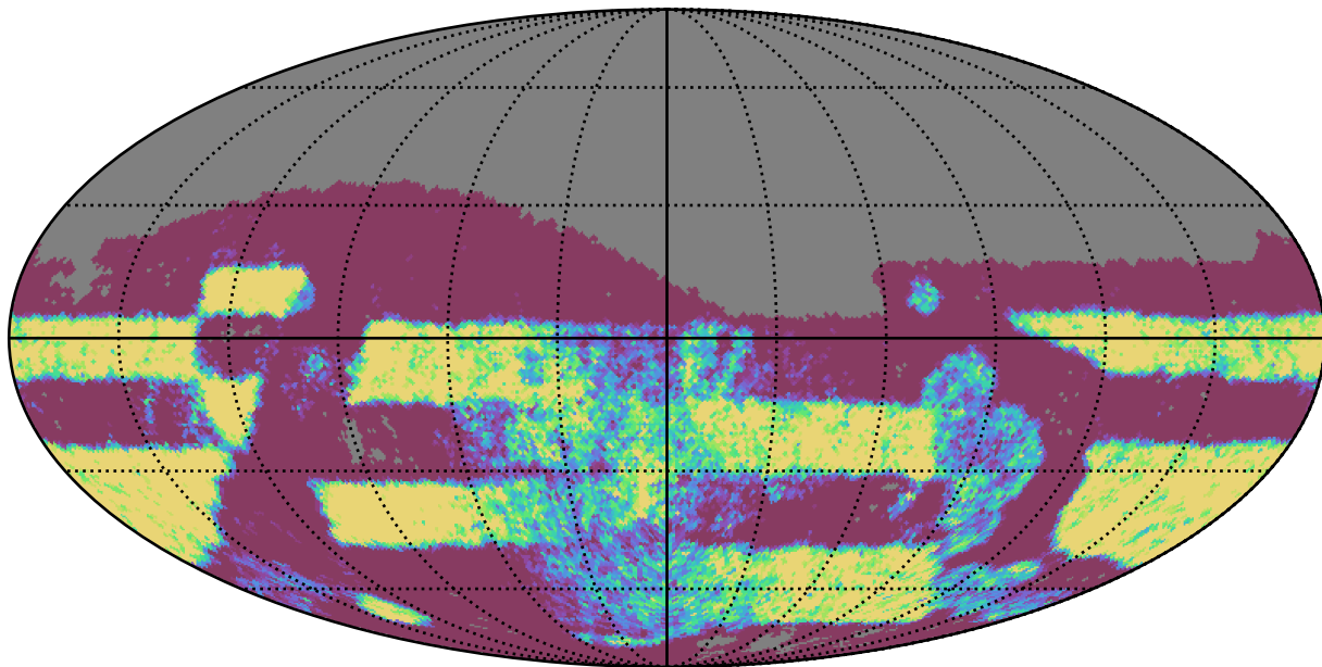
ddf_loaded_half_fl15_v3.4_10yrs Yr 3-4 i band: NVisits
