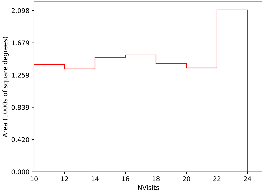
ddf_loaded_half_fl15_v3.4_10yrs Yr 3-4 i band: NVisits
