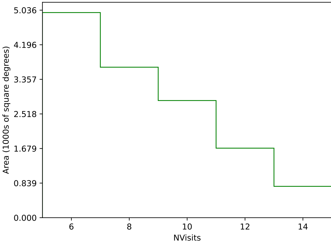
ddf_loaded_half_fl15_v3.4_10yrs Yr 3-4 g band: NVisits
