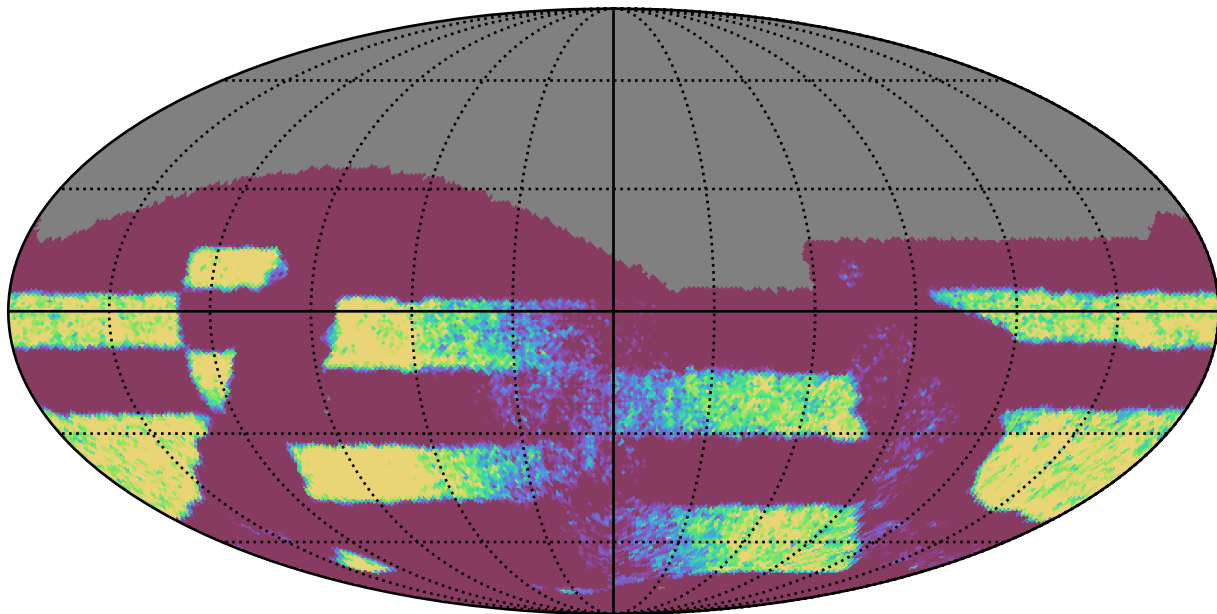
ddf_loaded_half_fl15_v3.4_10yrs Yr 3-4 all bands: NVisits
