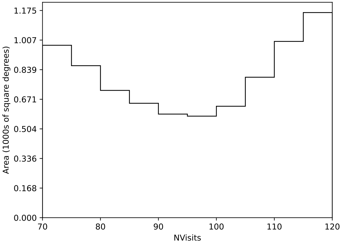
ddf_loaded_half_fl15_v3.4_10yrs Yr 3-4 all bands: NVisits
