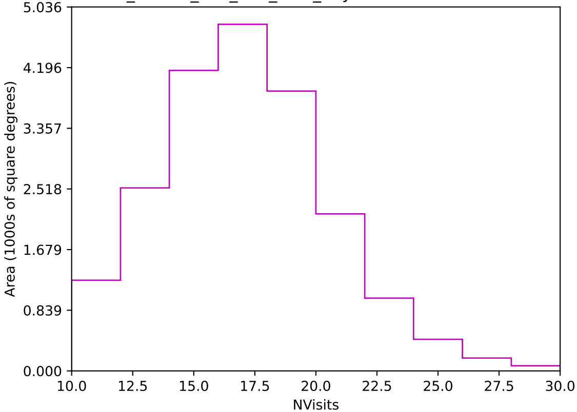
ddf_loaded_half_fl15_v3.4_10yrs Yr 1 z band: NVisits
