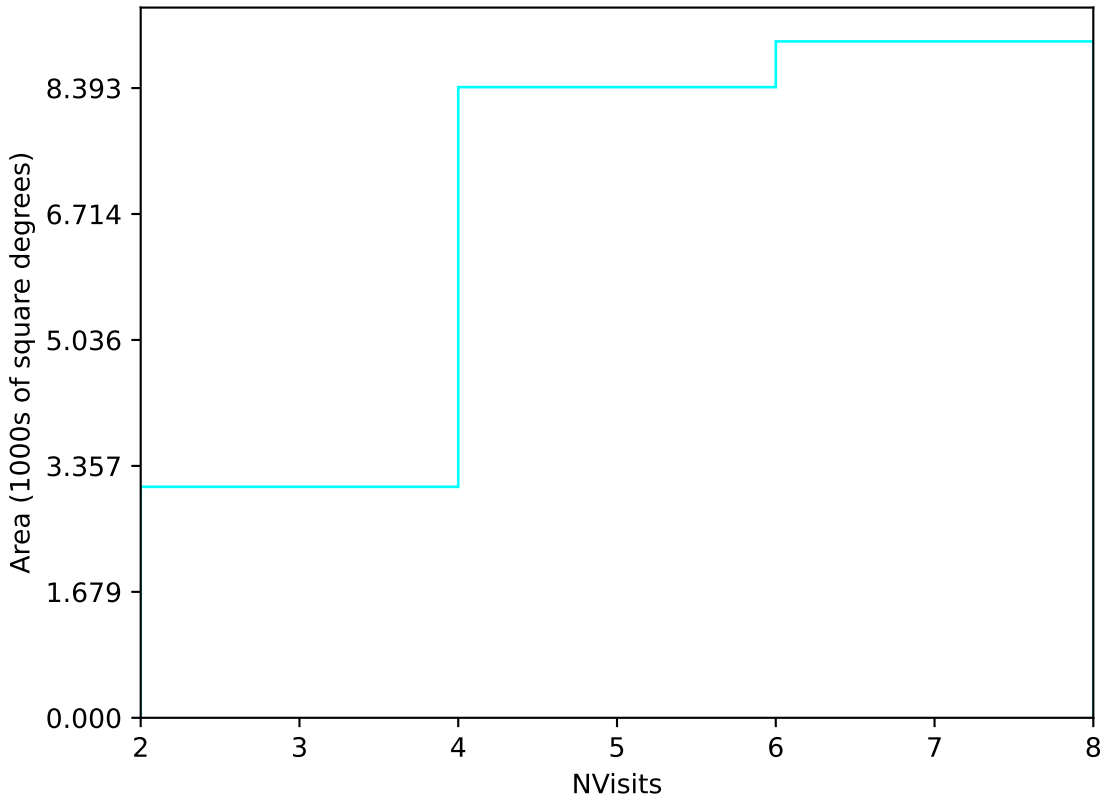
ddf_loaded_half_fl15_v3.4_10yrs Yr 1 u band: NVisits
